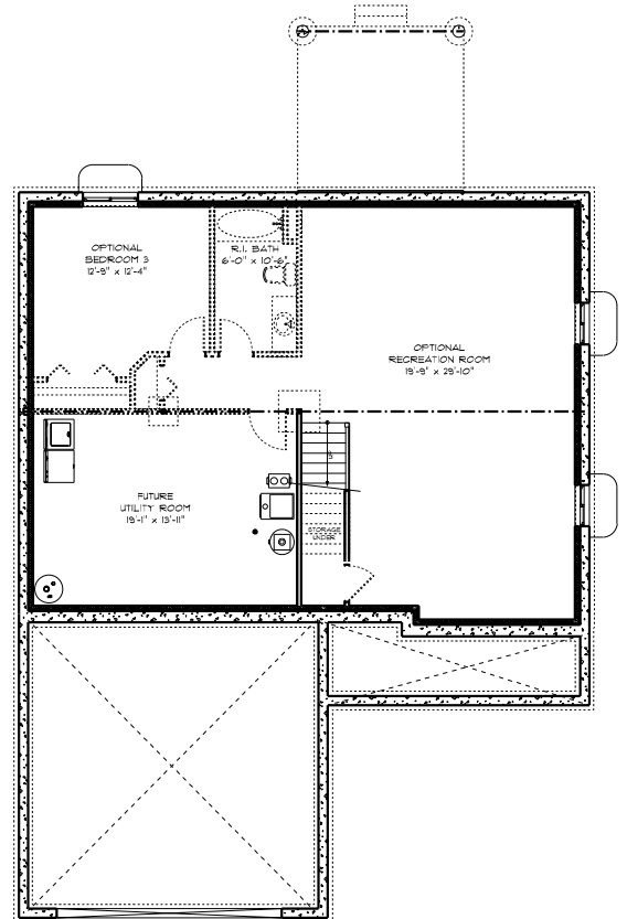
FOUNDATION PLAN
