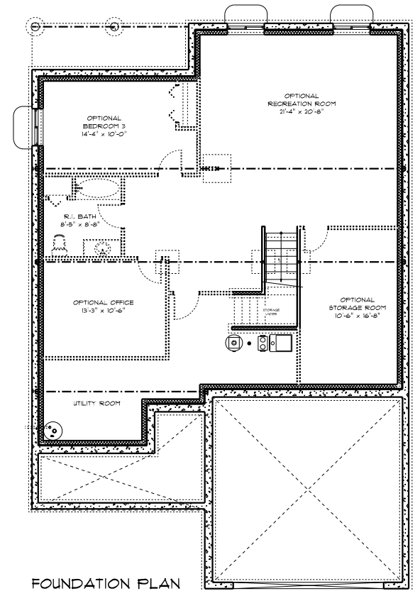
FOUNDATION PLAN 40'-8" x 61'-0"
