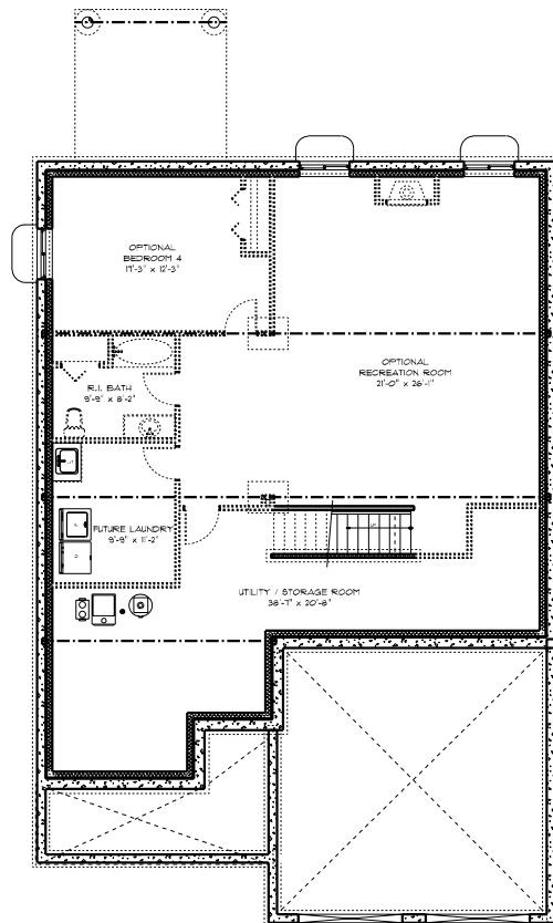
FOUNDATION 41'-0" x 60'-3"
