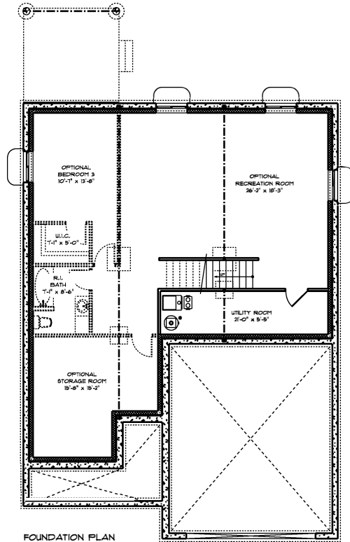
FOUNDATION PLAN 39'-6" x 54'-9"
