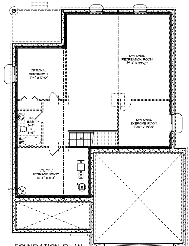
FOUNDATION PLAN 41'-0" x 55'-11"
