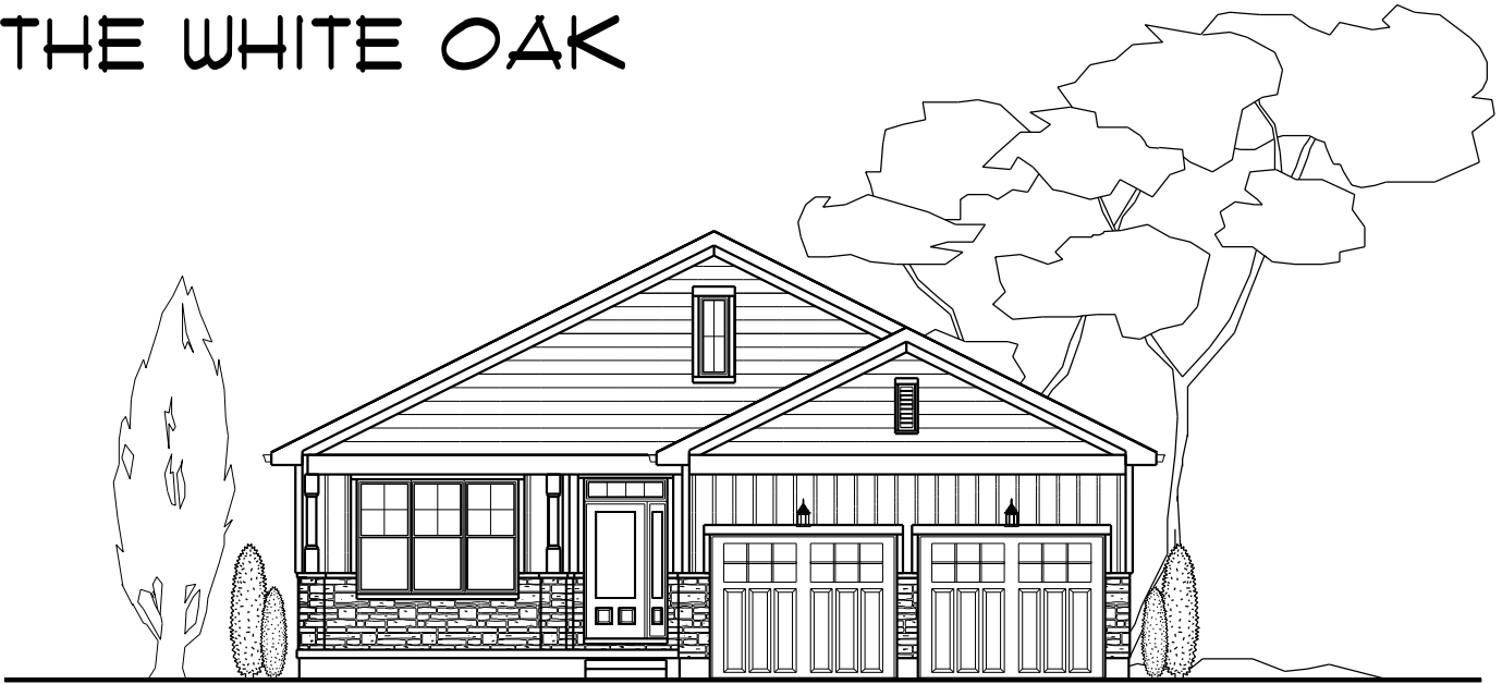
FRONT ELEVATION
