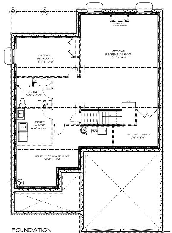
FOUNDATION 41'-0" x 60'-3"
